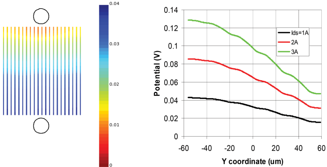
Potential distribution in source net and its 1D cross-section for different current levels can be used to easily identify the points in M1 and M2 layouts for measuring or sensing large area device current.
