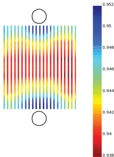
Distribution of V_{ds} (and I_{ds} ) over the power device area provides qualitative and quantitative estimate on design balance.
