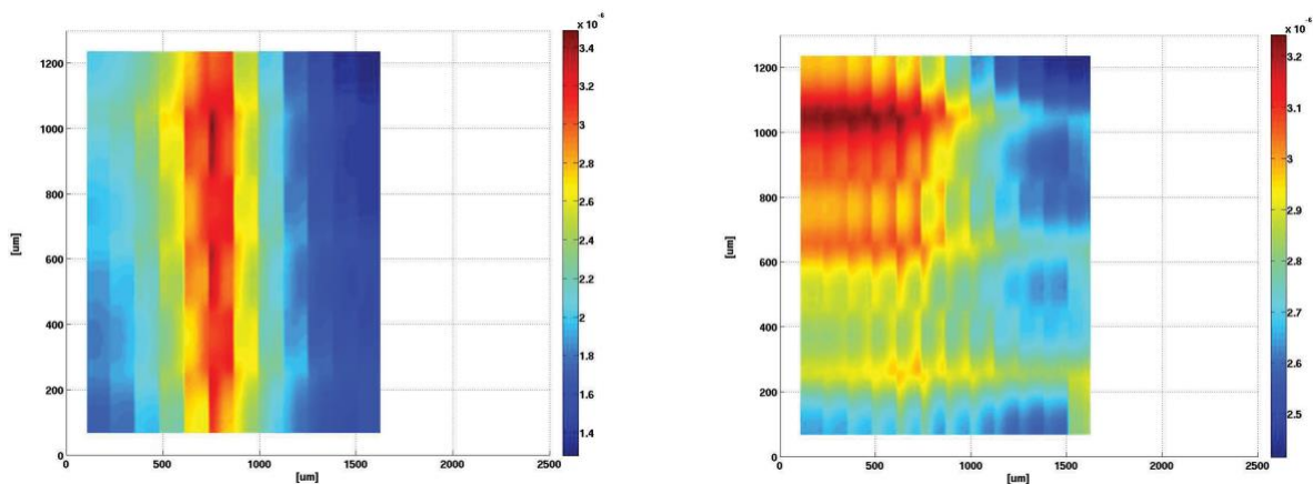
Visualization of I_{ds} through device (before and after modification) shows how adding more vias between two top metal layers lead to more uniform V_{ds} and I_{ds} distribution over device area.
